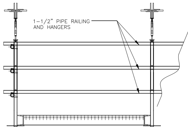
Typical hanger and railing system
